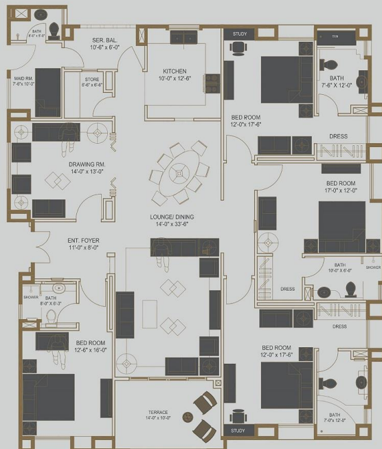
Ground to 11th Floor Plan
